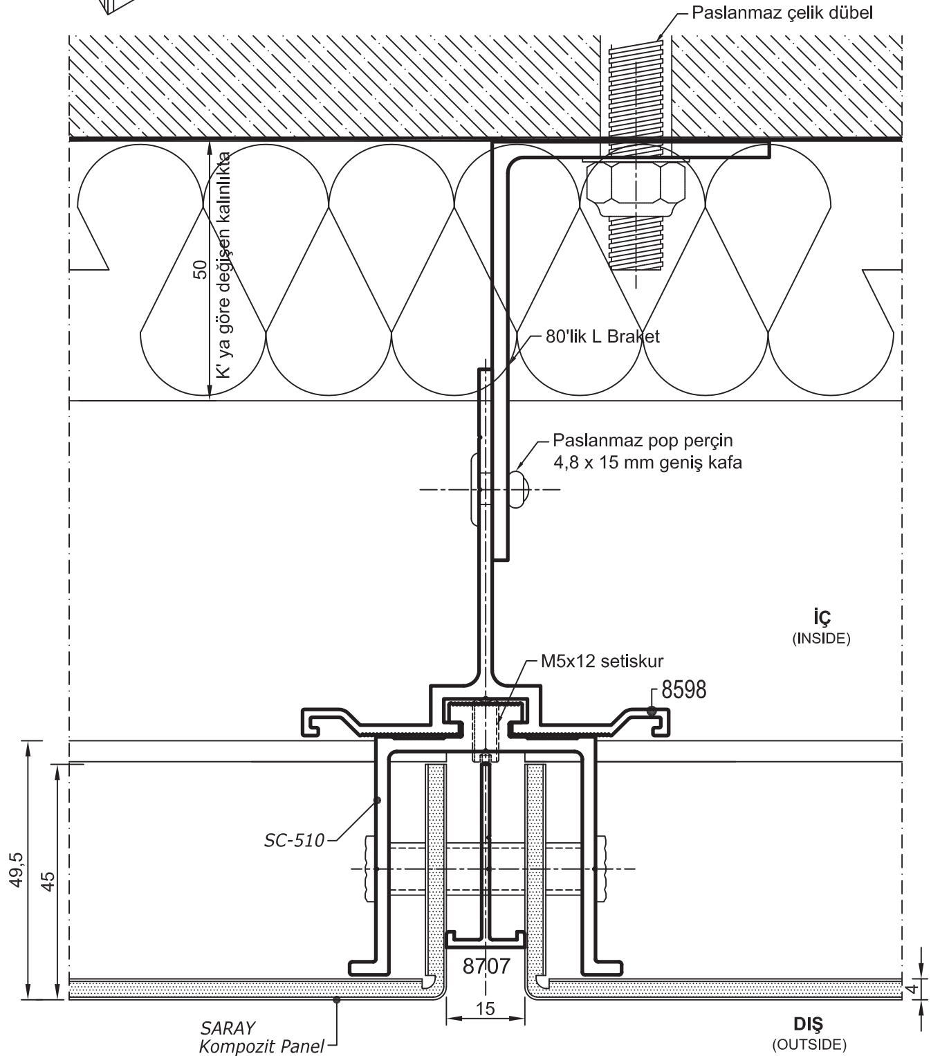
Detay Detail 1
