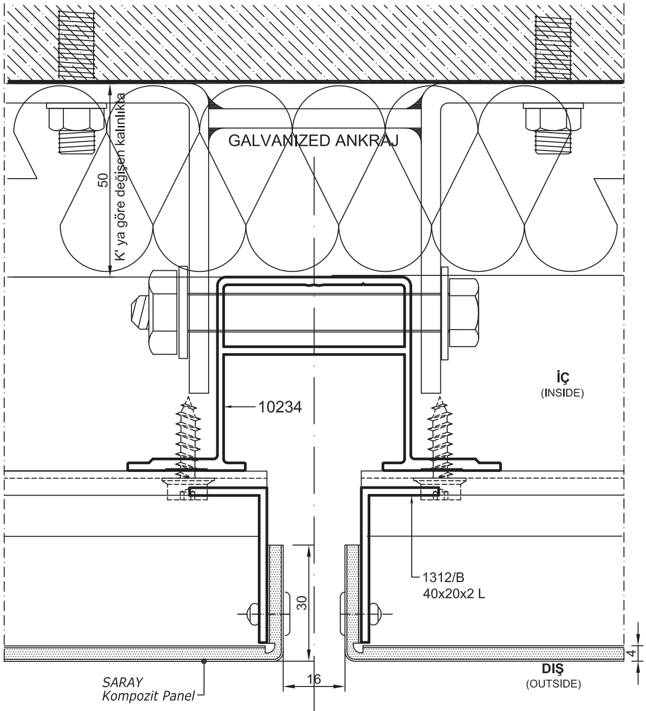
Detay 5 Detail 5
